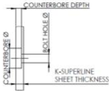
COUNTERBORE HOLE SCALE 1:1
